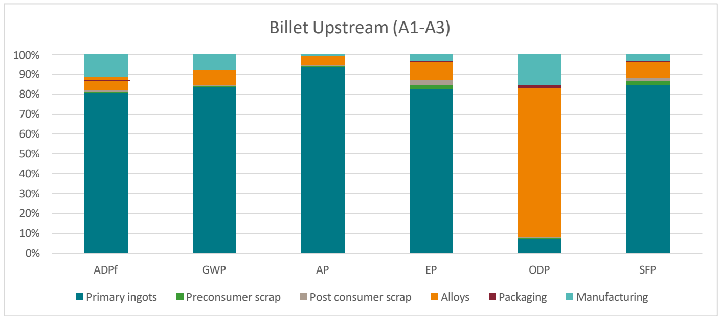
Figure 2. Relative contribution to upstream process
