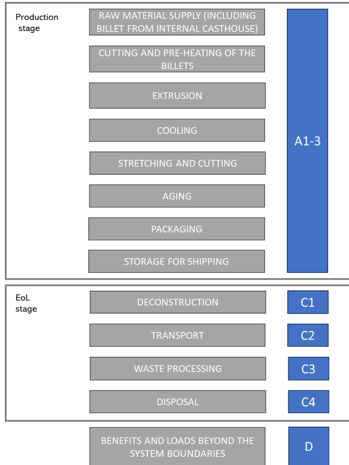
Figure 1. Scheme of the extrusion manufacturing process occurring at Spanish Fork
